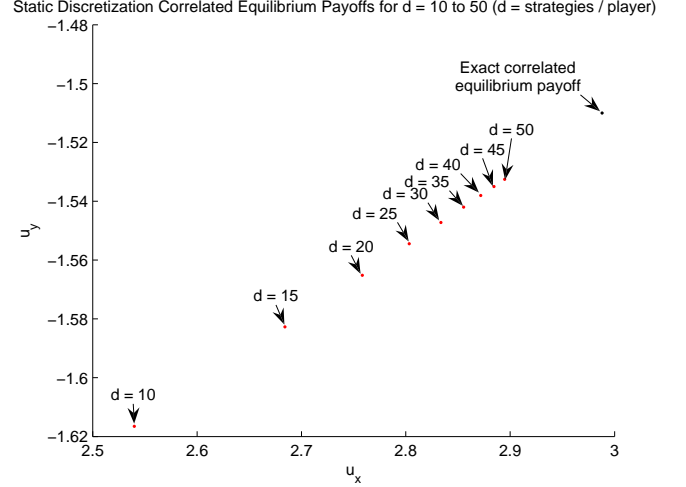
Fig. 1. Convergence of a sequence of \epsilon -correlated equilibria of the game in Example 3.1 computed by a sequence of static discretizations, each with some number d of equally spaced strategies chosen for each player. The axes represent the utilities received by players x and y . It can be shown that the convergence in this example happens at a rate \Theta(\frac{1}{d}) .
